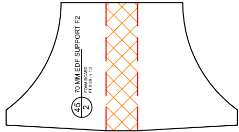
45 70 MM EDF SUPPORT F2 FOAM BOARD FT X-29 - v.1.0 2
