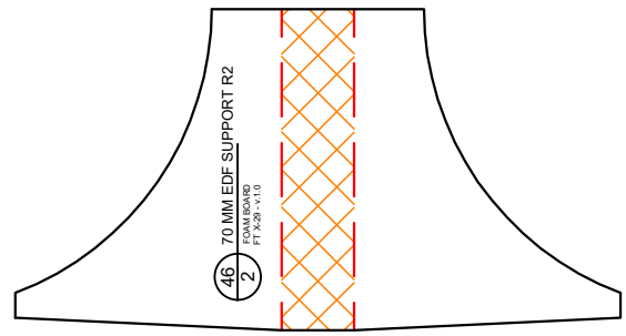
46 70 MM EDF SUPPORT R2 2 FOAM BOARD FT X-29 - v.1.0
