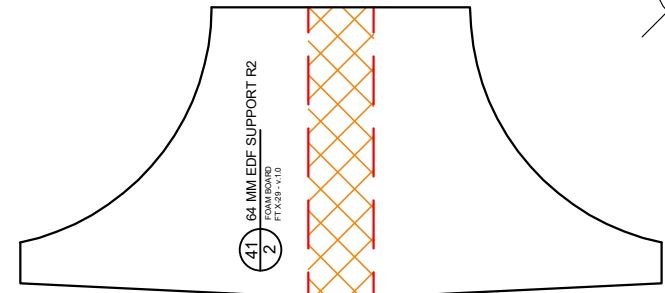
41 64 MM EDF SUPPORT R2 2 FOAM BOARD FT X-29 - v.1.0
